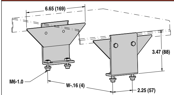
Cleated Stand Mounting Bracket
