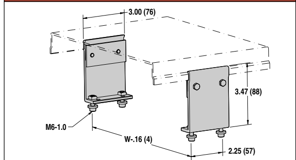
Flat Belt Stand Mounting Bracket
